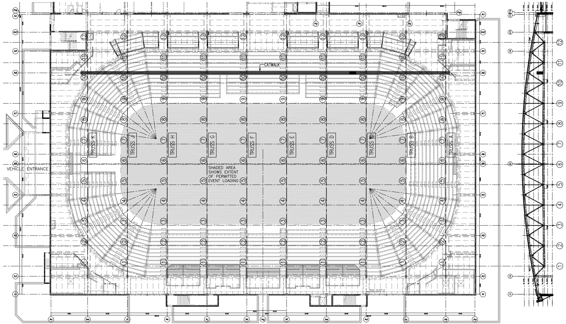
SEATING & TRUSS OVERLAY KEY PLAN SCALE N.T.S.
