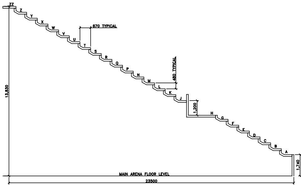
SIDE ELEVATION
