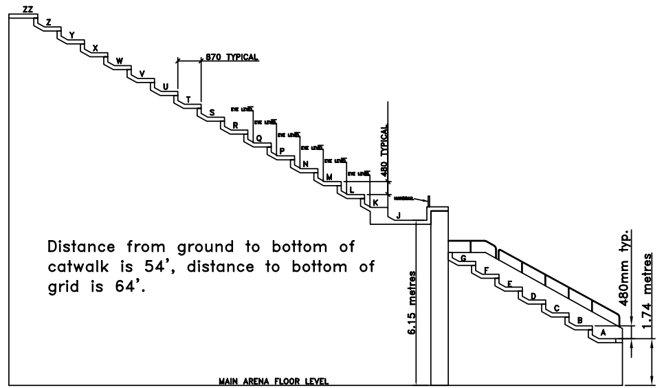
PROP STORE ELEVATION
